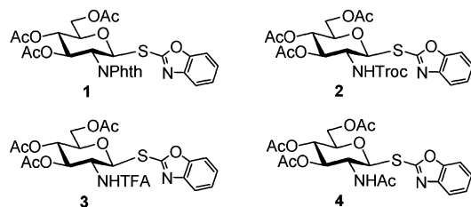
FIGURE 1. Differently N -substituted SBox glycosyl donors.
